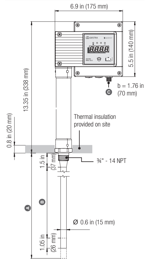
Fig. 2 A Maximum electrode length at 460 °F (238 °C) B Measuring range see table Fig. 1
