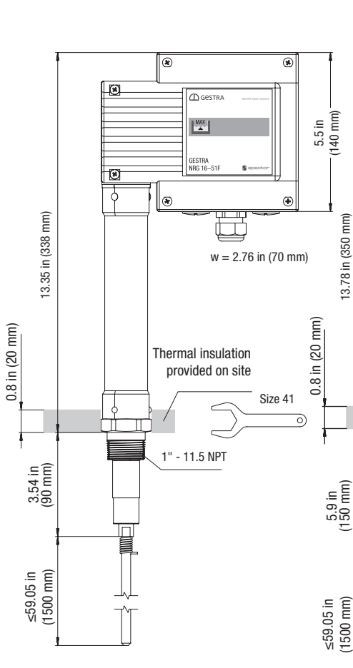
Fig. 9 NRG 16-51F, NRG 17-51F
