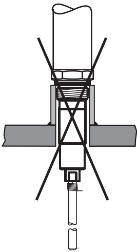
Fig. 13 NRG 16-51 NRG 17-51 NRG 19-51
