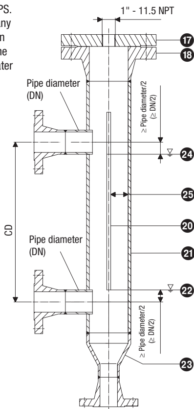
Fig. 19 Level pot if electrode is used as an external high-level alarm
