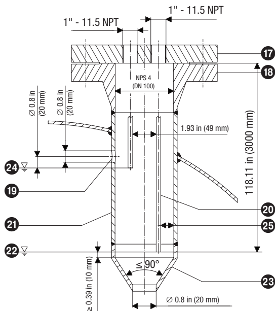
Fig. 18 Protective tube (provided on site) if electrode is used as an internal water level limiter combined with level control or high-level alarm
