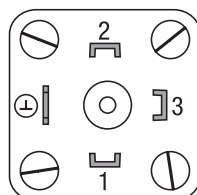
Fig. 22 Connecting the level electrode with four-pole connector
