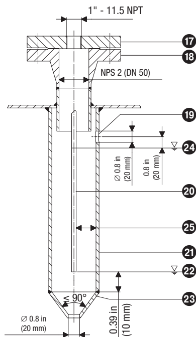
Fig. 17 Protective tube (provided on site) if electrode is used as an internal water level limiter
