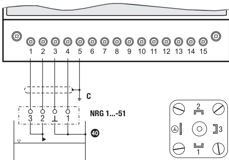
Fig. 22 Connecting the level electrode with four-pole connector
