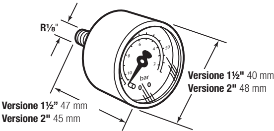
Dimensioni (approssimative) in millimetri
