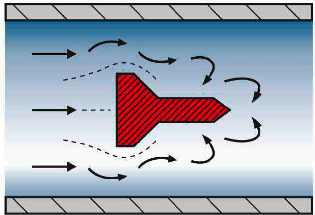
Vortex body with integrated baffle
