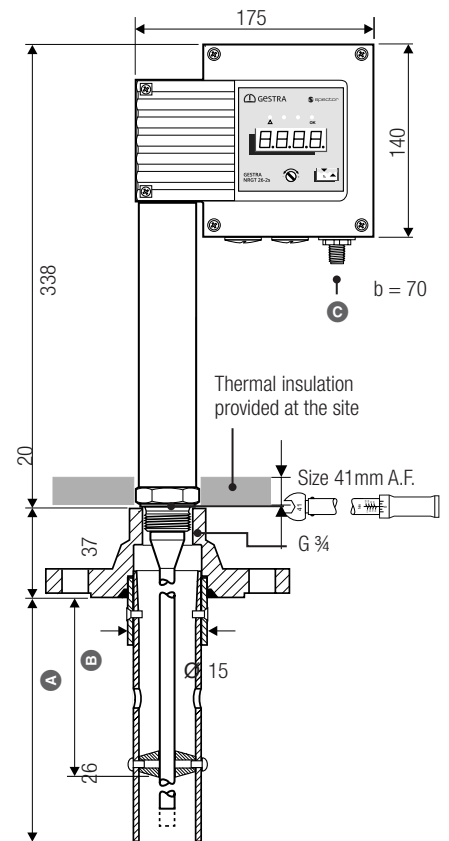
Fig. 2 A Maximum electrode length at 238 °C B Measuring range See table in Fig. 1
