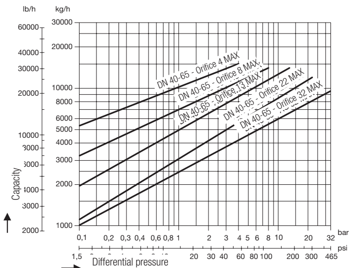
Capacity chart of UNA 47 MAX with cold water
