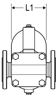
Horizontal installation
