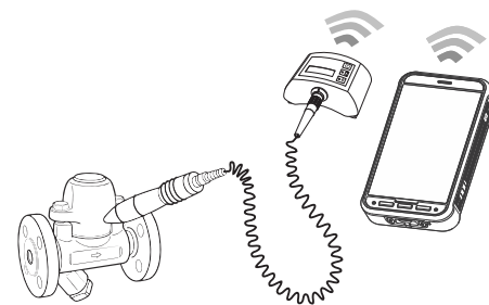
Testing the steam trap
