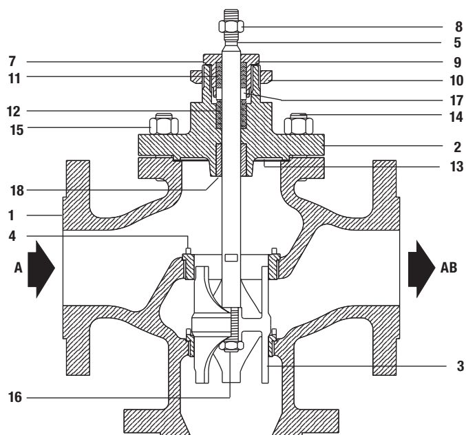
QLM Mixing valve
