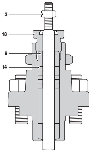
KE valve with graphite packing
