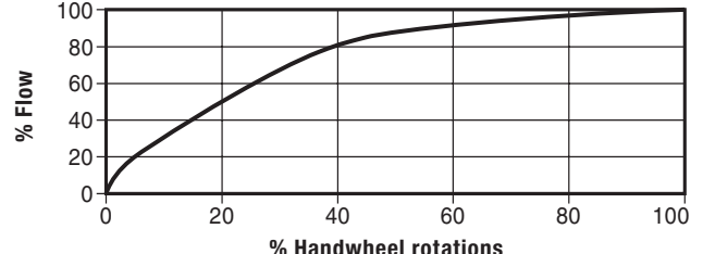
Typical standard flat disc for the GAV 63F, GAV 64F, GAV 65F and GAV 66F
