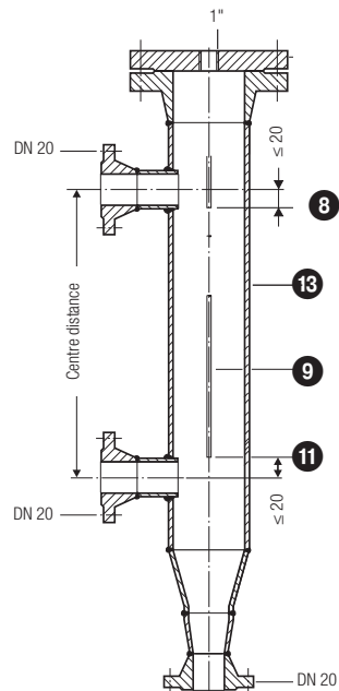
Fig. 3 Level pot DN 80 for external installation
