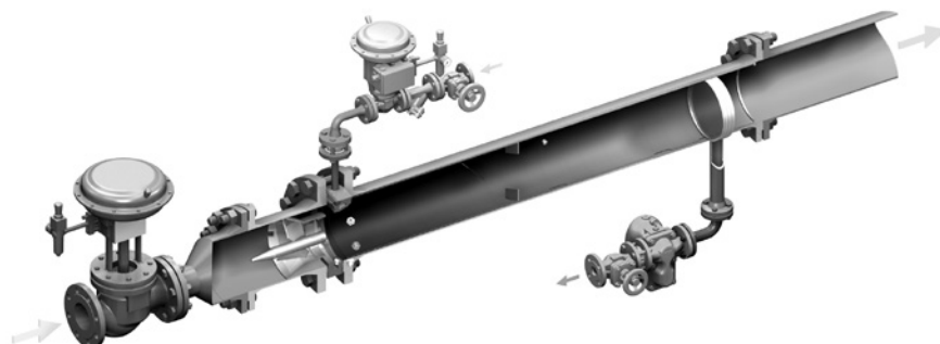
Injection cooler EK, sectional view
