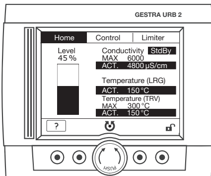
URB 2 Home screen (steam boiler)
