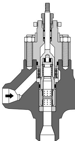
Special nozzle Δp max 370 bar/5365 psi
