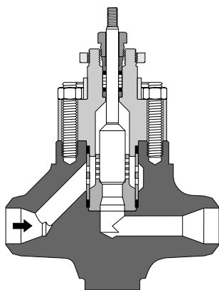
Special nozzle without tandem seat Δp max 40 bar/580 psi
