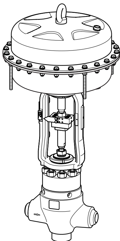
ZK 313-D/20 1" – 3"
