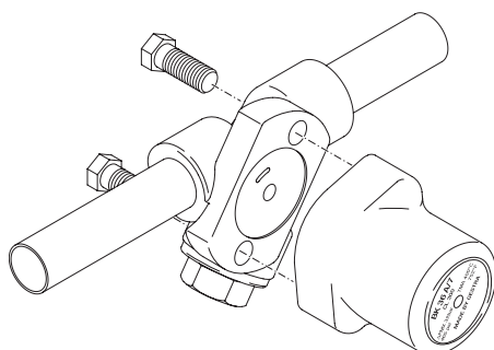
Steam trap unit attached to universal connector
