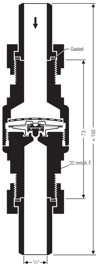
Design with union butt-weld nipples
