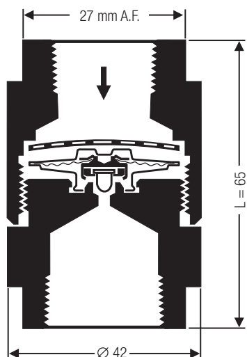
Design with screwed sockets
