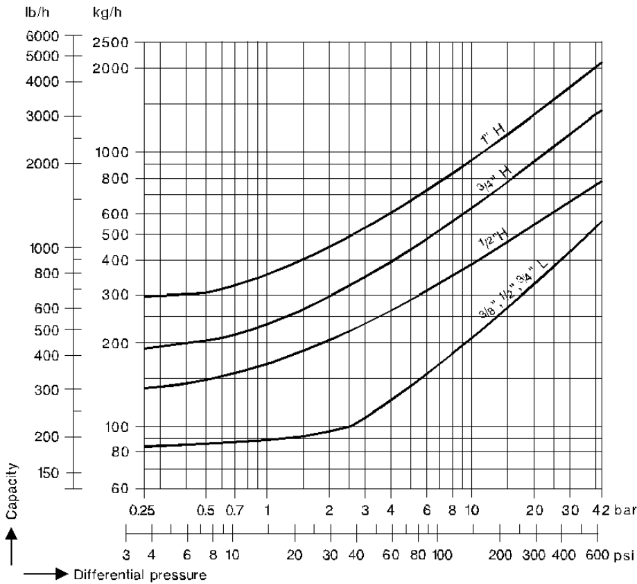
Capacity Chart DK 57
