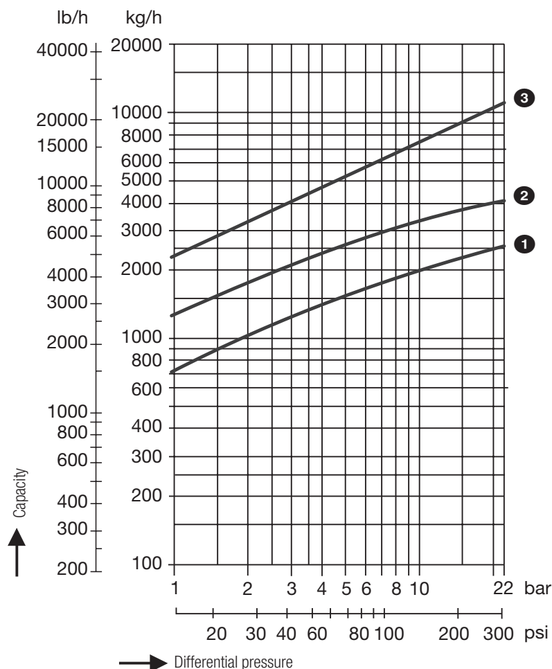
Capacity chart
