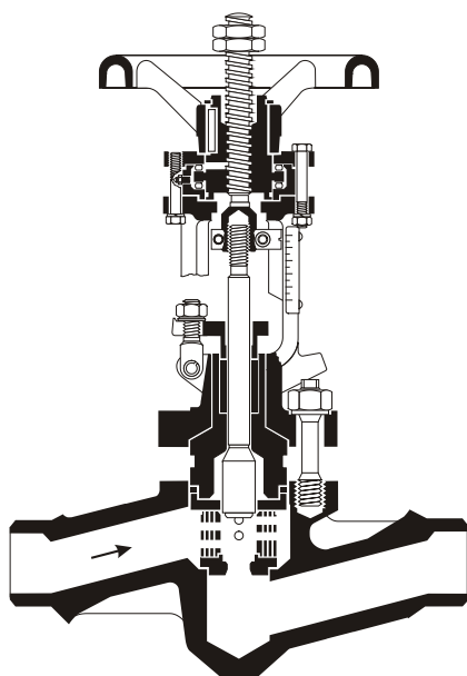
ZK 210/02, DN 50 (2") with butt-weld ends
