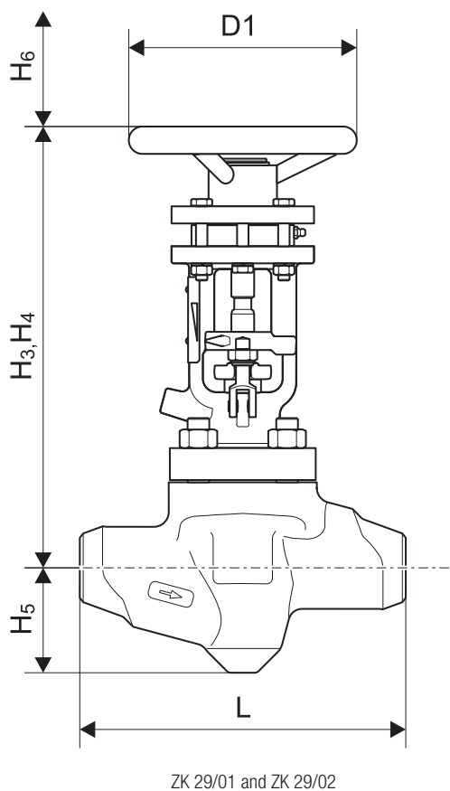
Dimensions [mm]
