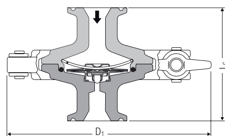
SMK 22 with joint clamp and clamp connections
