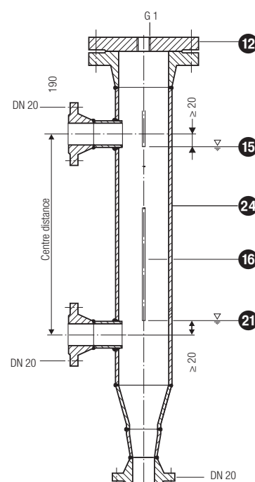
Fig. 6 External level pot
