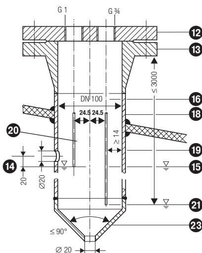
Fig. 5 Protection tube (provided on site) for installation inside the boiler and in combination with other GESTRA equipment
