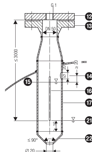
Fig. 4 Protection tube (provided on site) for installation inside the boiler
