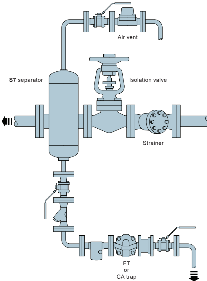
Fig. 8 Separator on a steam line
