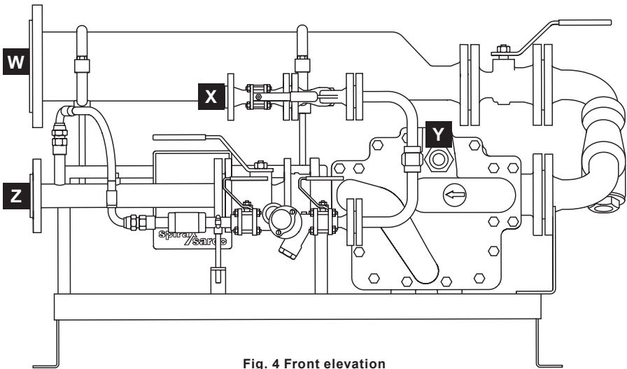
Fig. 4 Front elevation
