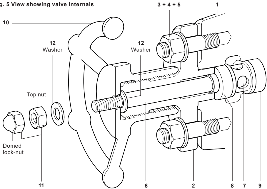
Fig. 5 View showing valve internals
