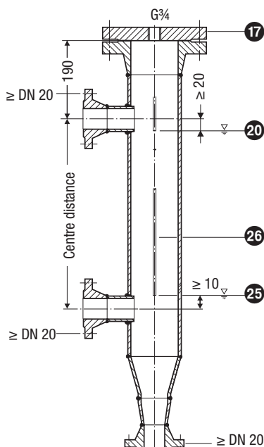
Fig. 18 Level pot \geq \text{DN } 80 if electrode is used as external water level limiter
