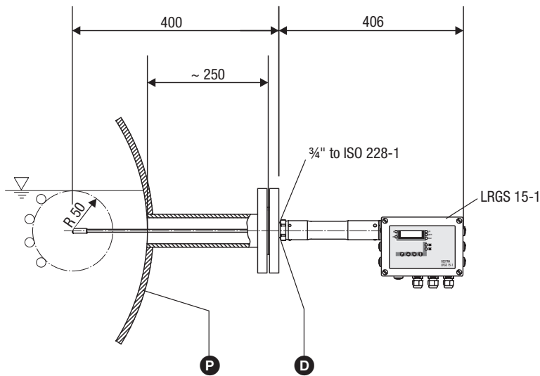
LRGS 15-1 used as conductivity electrode
