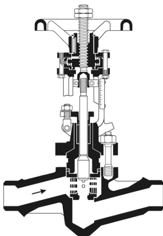
Control valve ZK 210-D/14 DN 25 with handwheel
