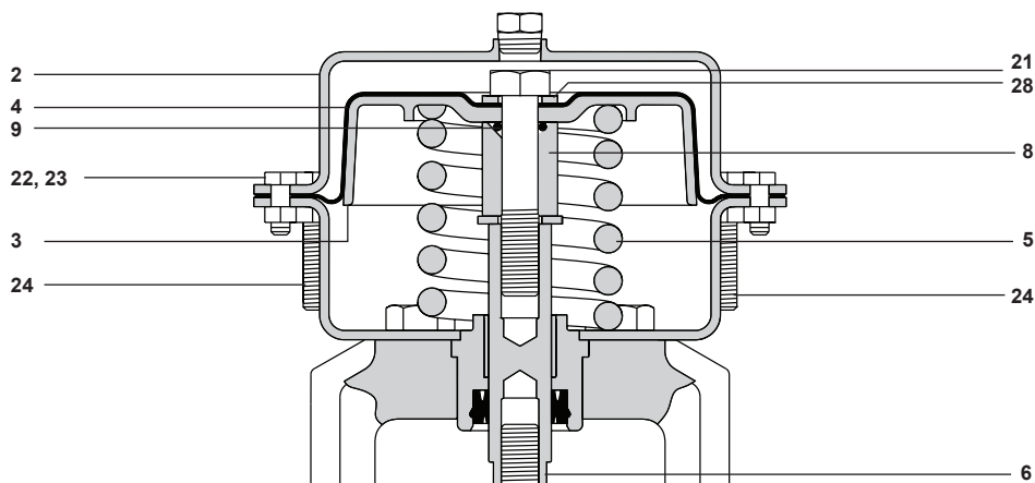
Abb. 16 PN9100R
